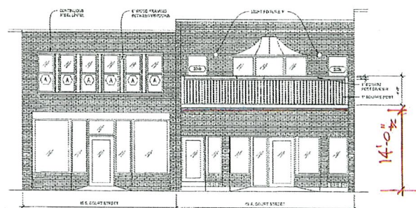
A AB FRONT BUILDING ELEVATION 1/4" = 1' - 0"
