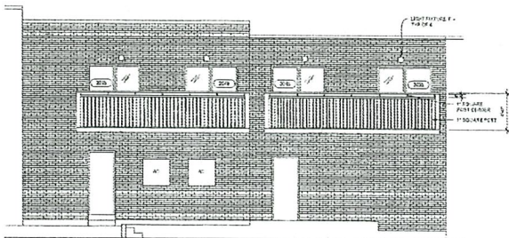
B AB REAR BUILDING ELEVATION 1/4" = 1' - 0"
