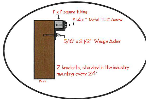
Mounting Detail (Brick Wall)
