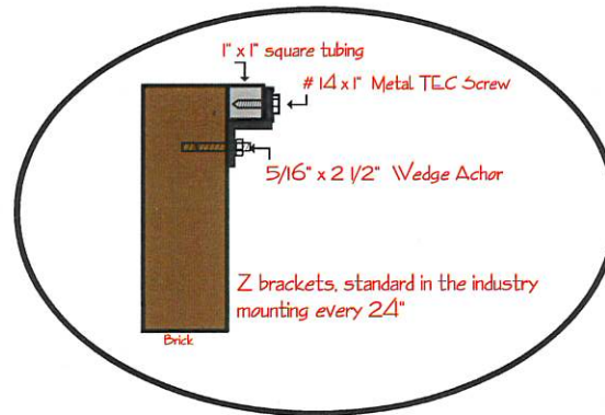
Mounting Detail (Brick Wall)
