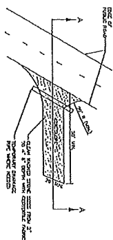
PLAN VIEW OF TEMPORARY CONSTRUCTION ROAD
