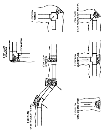
TYPICAL CONCRETE THRUST BLOCKING
